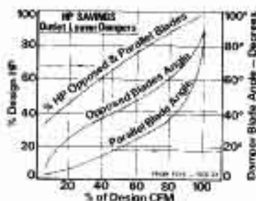
Fig. 4 H.P. Savings
