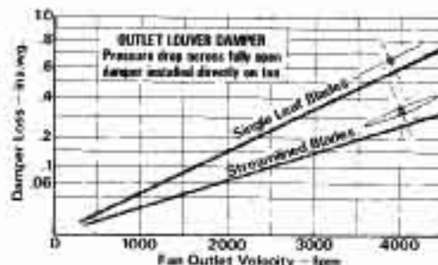
Fig. 5 Damper Losses
